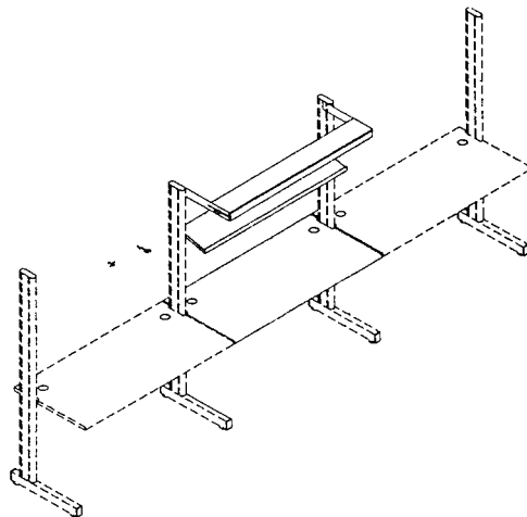
BRIDGE WORKSTATIONS WITH LIGHT AND SHELF ACCESSORY
